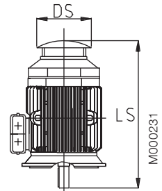
Protective roof, variant code 005
